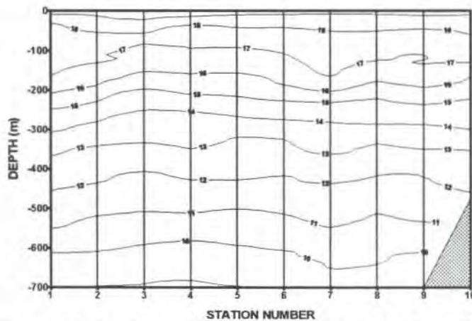
Figure A3. Section of XBT, South of ESTOC, May 1994; (Station 1 → 27.6N, 15.2W; Station 10 → 26.1N, 15.2W).
