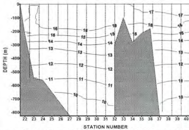
Figure A2. Section of XBT, North of ESTOC, April 1994; (Station 22 → 31.5N, 10.4W; Station 40 → 29.5N, 13.6W).
