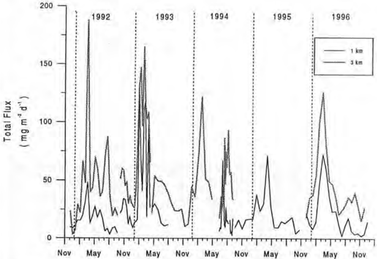
Figure 15. Total particle flux at ESTOC determined with particle traps at 1 km (thin line) and 3 km depth (thick line).
