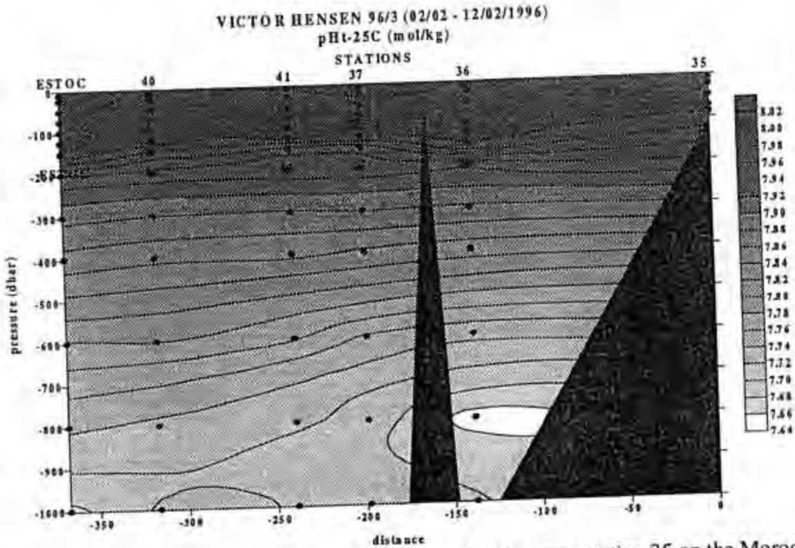
Figure 30. Spatial variability of the pHt in the section between station 35 on the Moroccan continental slope and ESTOC.
