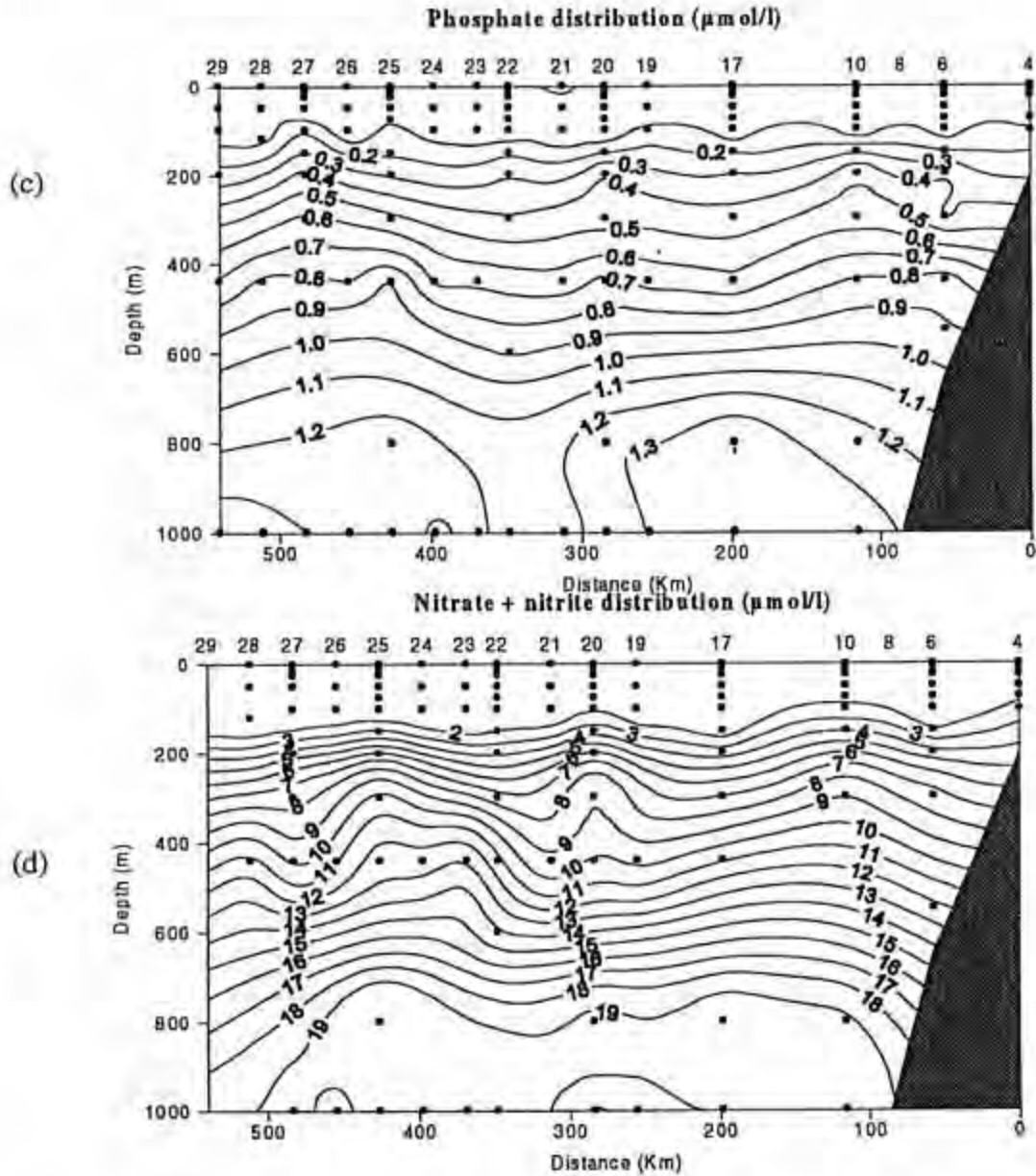
Figure 29 (c,d). Distributions of phosphates and nitrate+nitrite during FS "Victor Hensen" cruise VH 96-1 on the zonal section at about 29°N.
