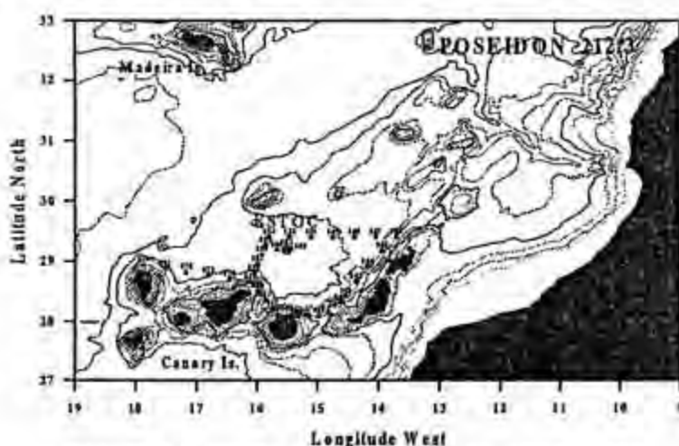
Figure 5. Stations sampled during cruise P212/3.
